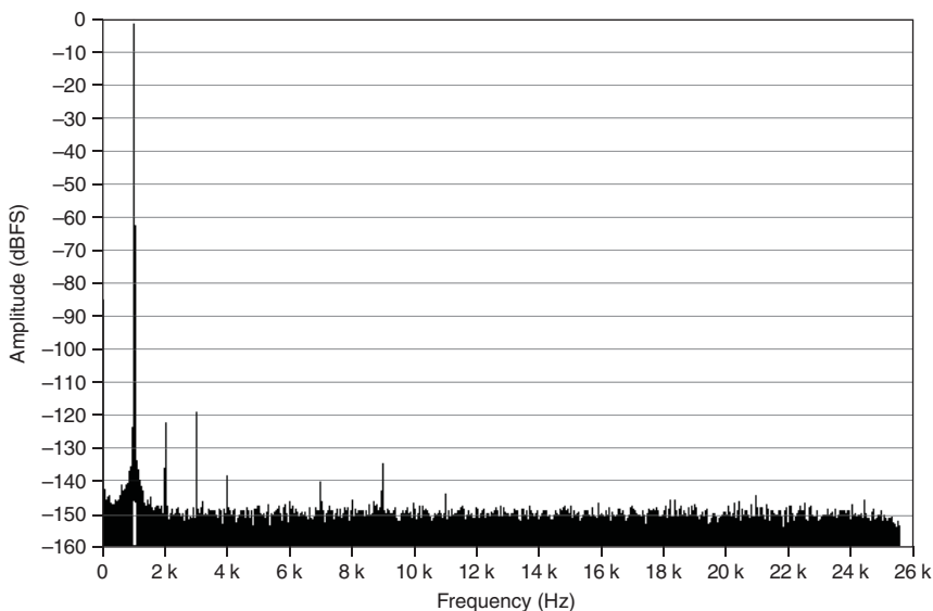
Figure 6. FFT of -1 dBFS, 1 kHz Tone Acquired at 51.2 kS/s, 10 dB Gain
