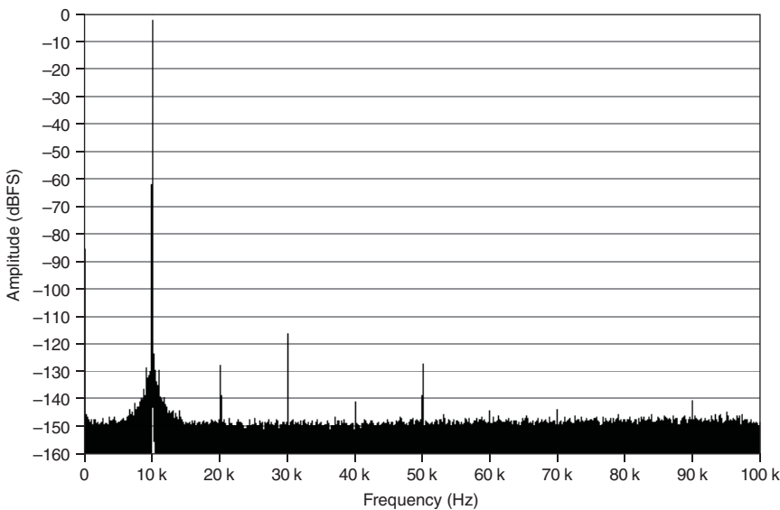
Figure 10. FFT of -1 dBFS, 10 kHz Tone Acquired at 204.8 kS/s, 10 dB Gain
