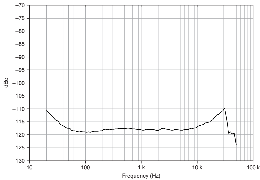
Figure 13. THD (0 dB Gain, Balanced Source, Differential Configuration, 204.8 kS/s)
