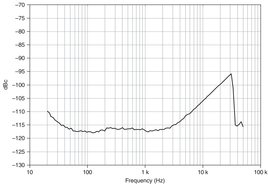
Figure 16. THD (30 dB Gain, Balanced Source, Differential Configuration, 204.8 kS/s)
