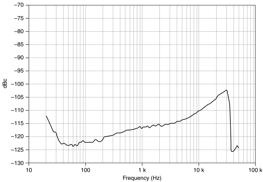
Figure 15. THD (20 dB Gain, Balanced Source, Differential Configuration, 204.8 kS/s)
