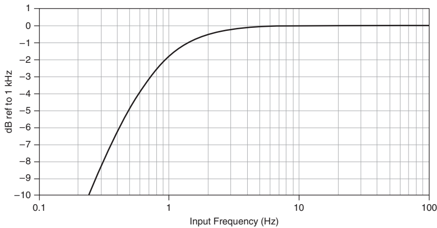
Figure 1. Magnitude Response of AC Coupling Circuit (Typical)
