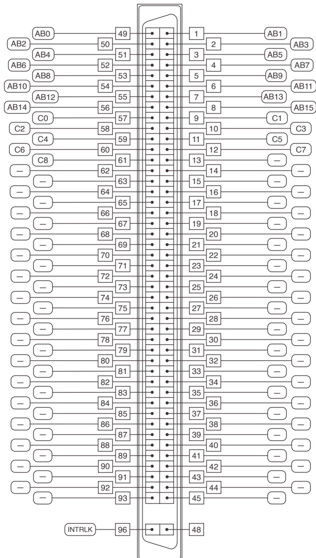
Figure 1. SWB-2812A/B Connector Pinout
