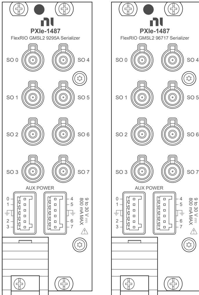
Figure 8. Serializer Front Panels
