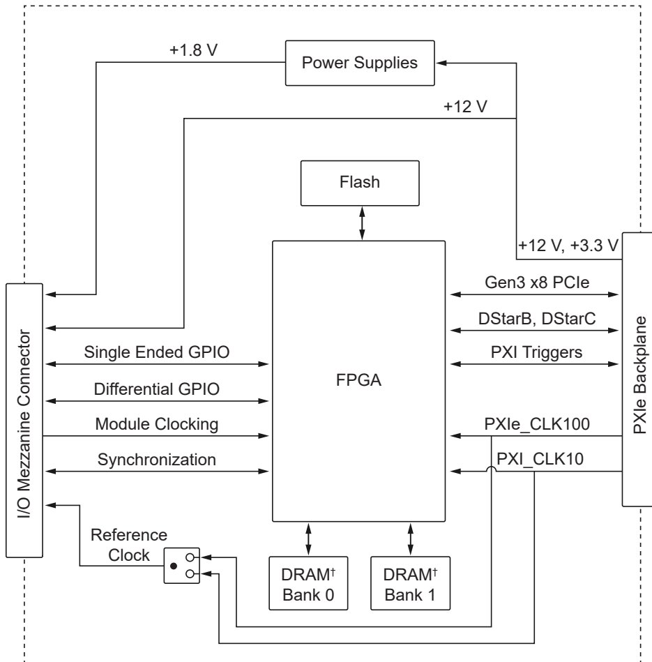
Figure 15. PXIe-1487 FPGA Block Diagram
