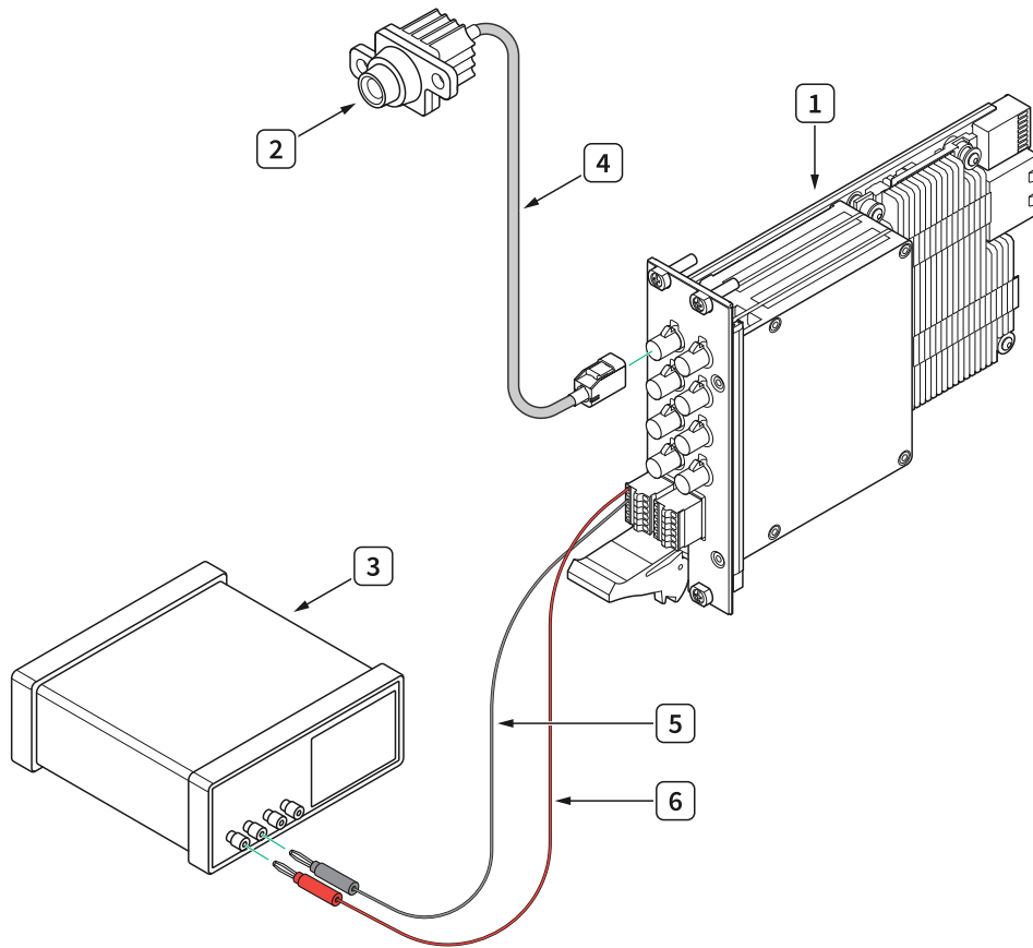
Figure 3. PXle-1487 Deserializer
