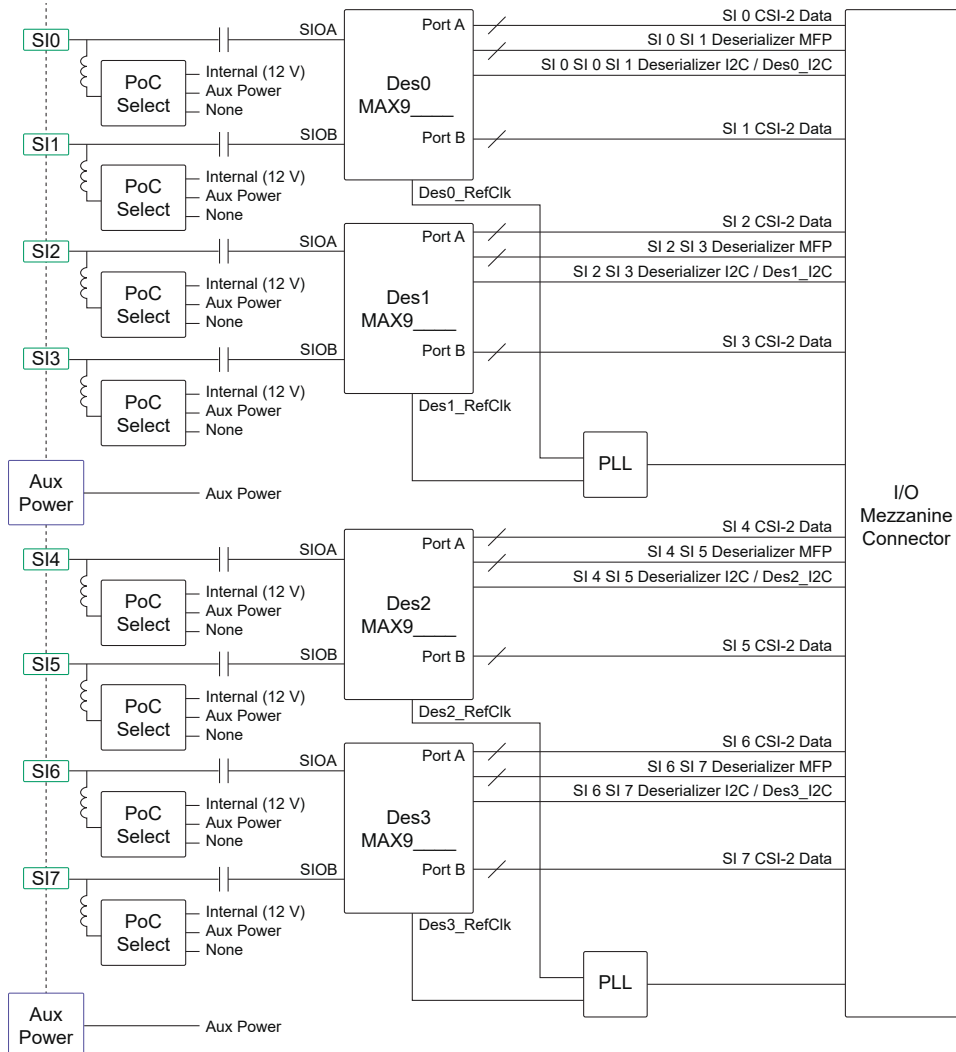
Figure 12. Deserializer Block Diagram
