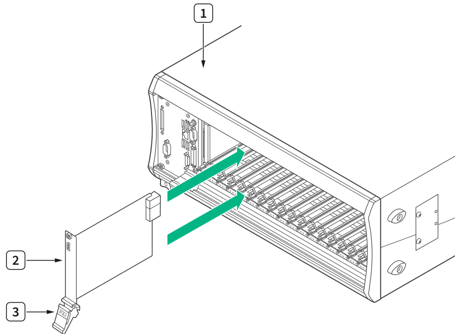
Figure 2. Module Installation
