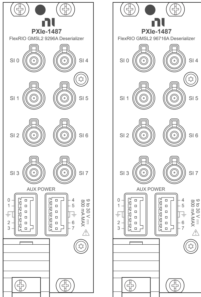
Figure 6. Deserializer Front Panels
