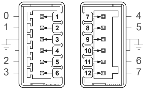
Figure 7. Deserializer AUX Power Connectors
