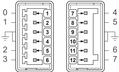
Figure 9. Serializer AUX Power Connectors
