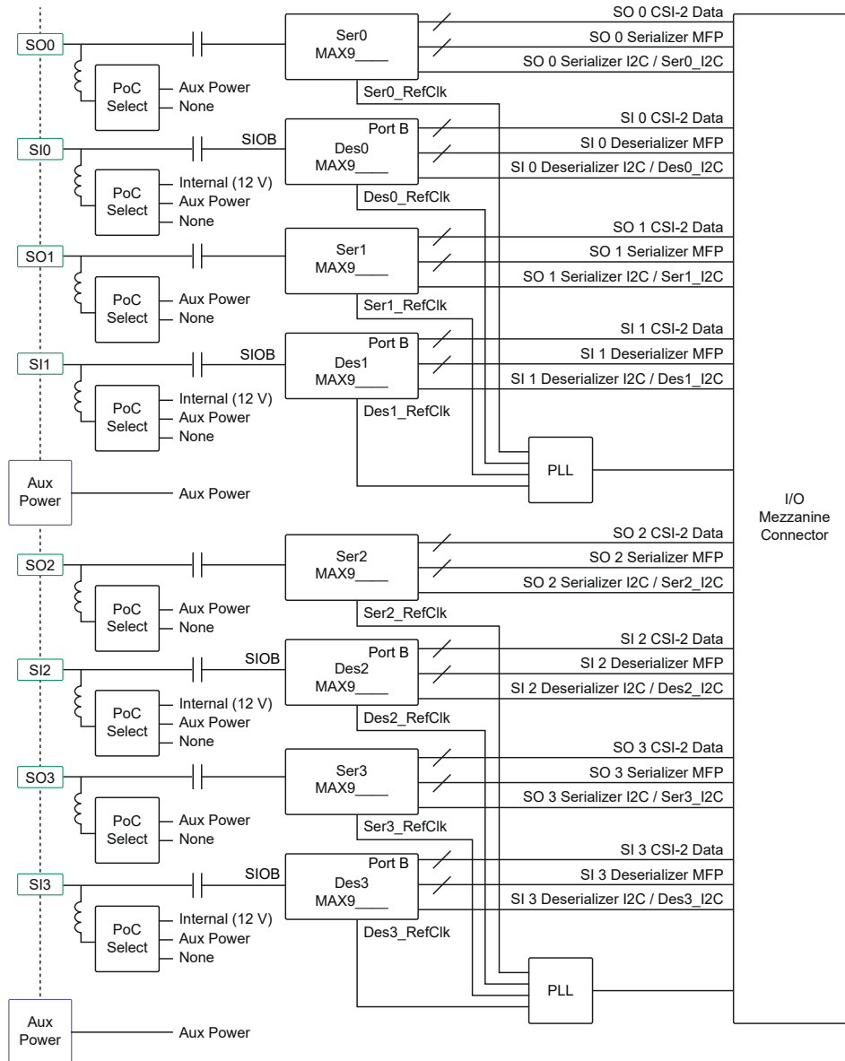
Figure 14. SerDes Block Diagram
