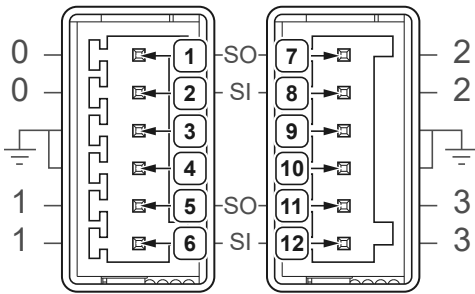
Figure 11. SerDes AUX Power Connectors
