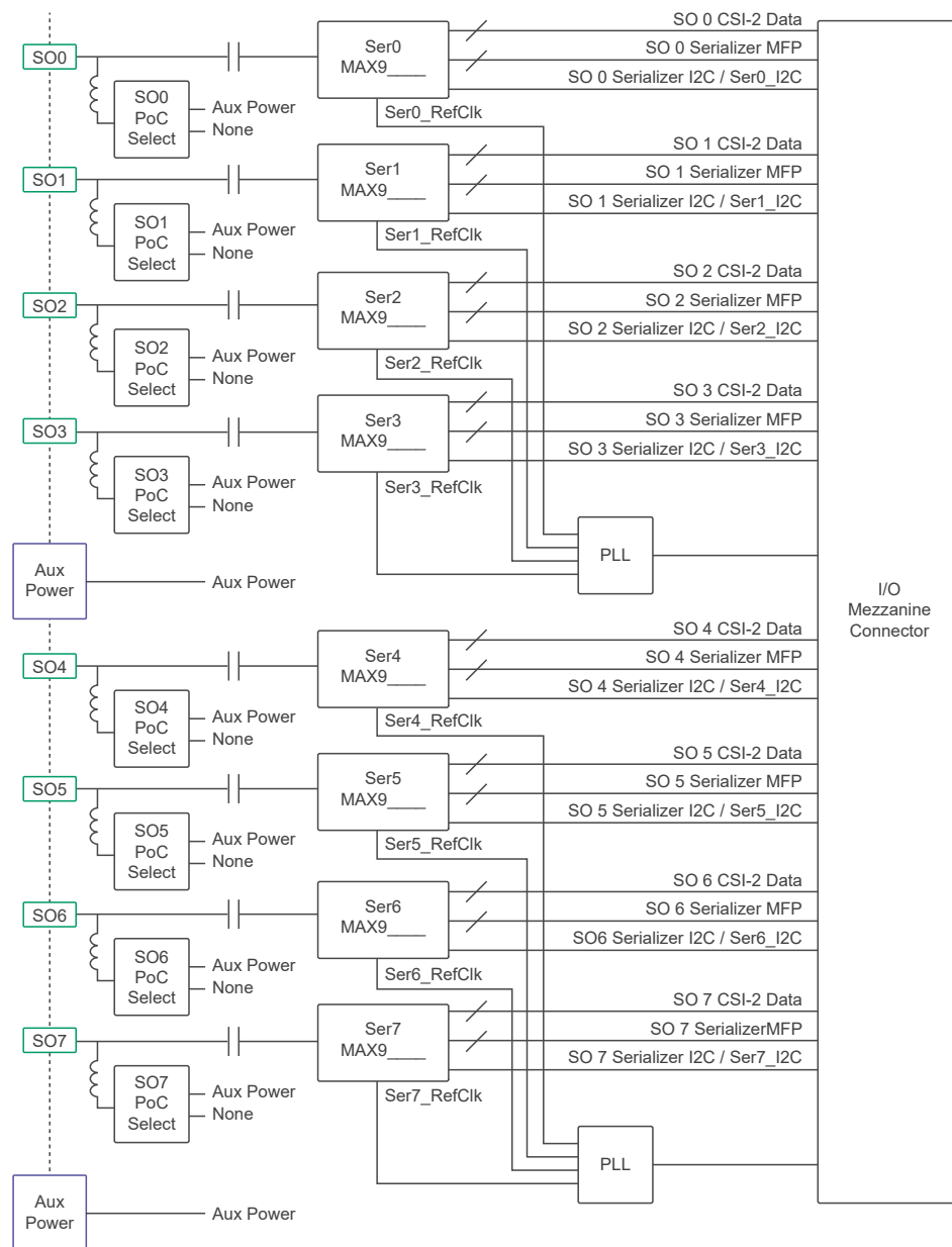
Figure 13. Serializer Block Diagram
