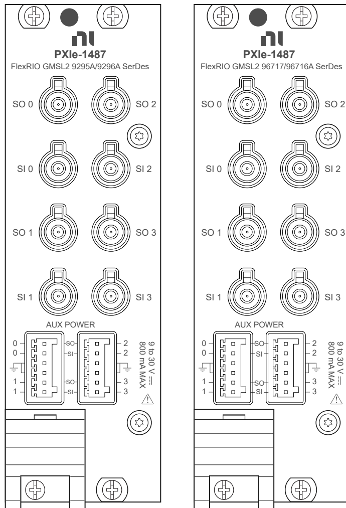
Figure 10. SerDes Front Panels
