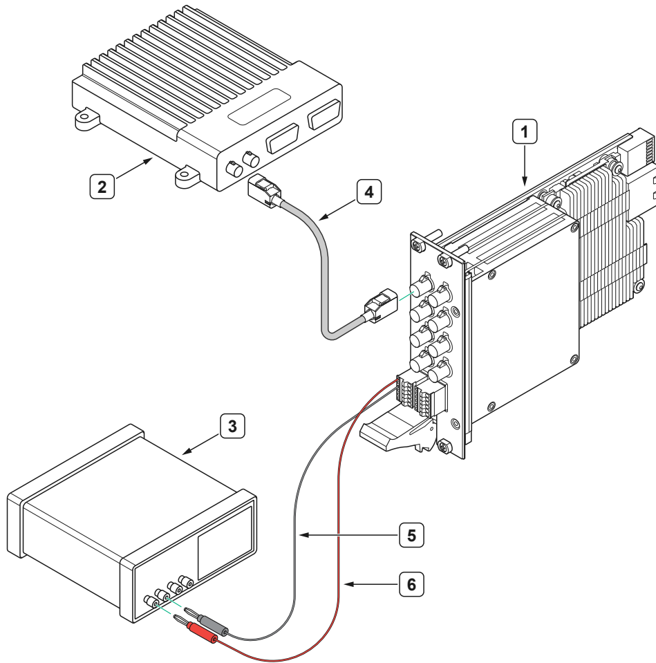
Figure 4. PXle-1487 Serializer
