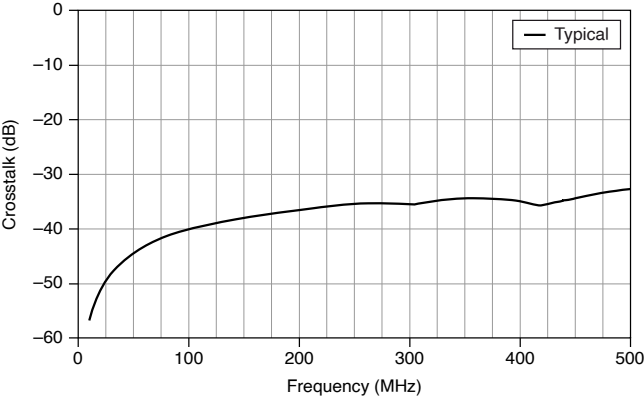
Figure 5. Crosstalk, Typical
