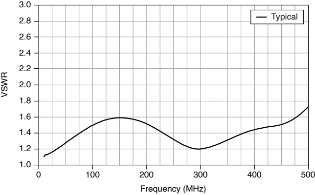
Figure 3. VSWR, Typical
