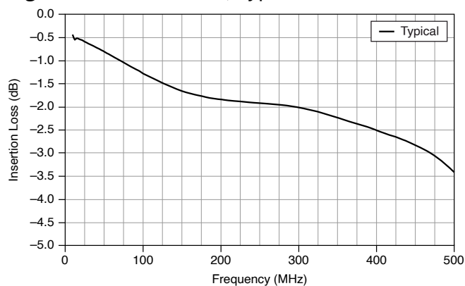
Figure 2. Insertion Loss, Typical
