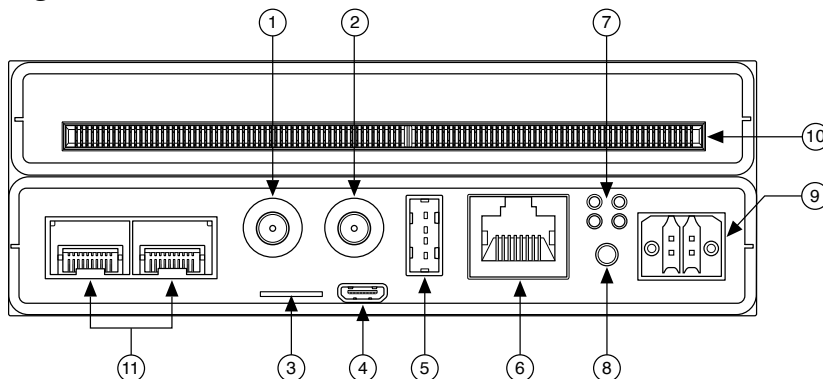
Figure 3. NI-7935
