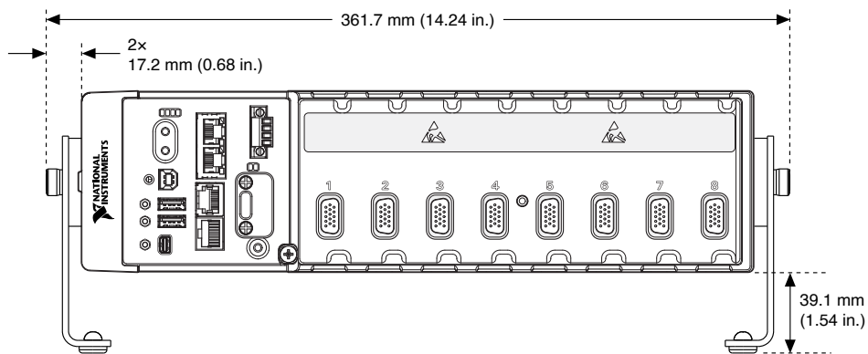
Figure 10. cRIO-9036 Desktop Mounting Front Dimensions
