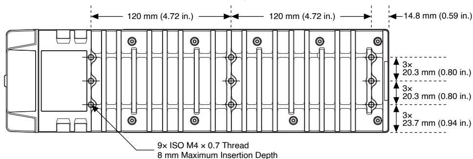
Figure 8. cRIO-9036 Surface Mounting Dimensions
