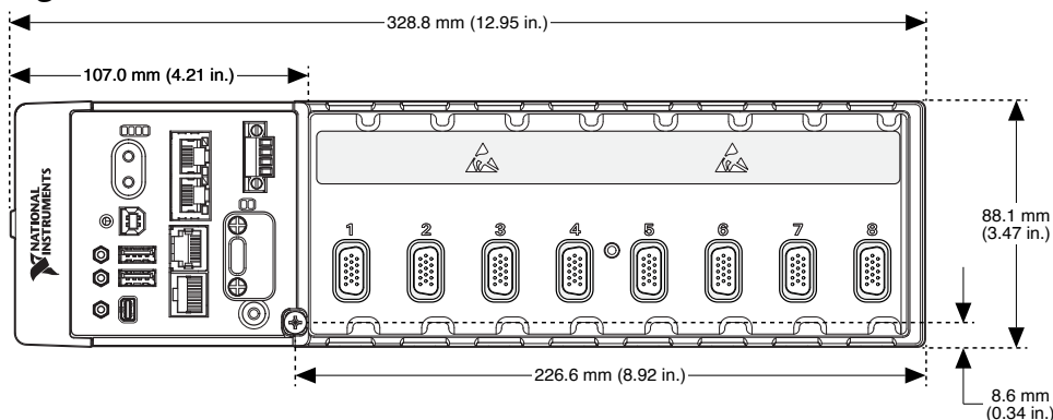
Figure 4. cRIO-9036 Side Dimensions
