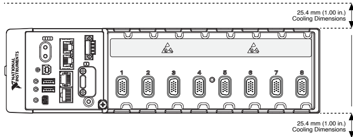
Figure 5. cRIO-9036 Cooling Dimensions
