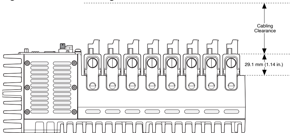
Figure 6. cRIO-9036 Cabling Clearance
