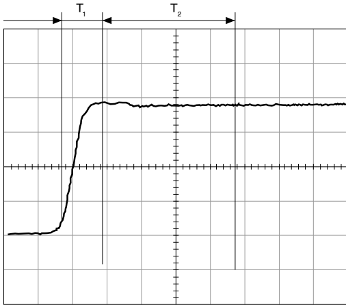
Figure 9. HF Compensation Trimmer
