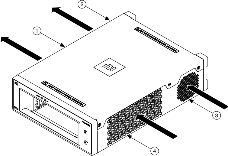
Figure 3. PXIe-1090 Cooling Air Flow
