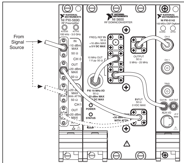
Figure 1. NI PXI-5690 RF Preamplifier Attached to NI PXI-5661 RF Vector Signal Analyzer
