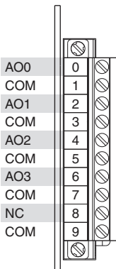
Figure 2. NI 9263E Terminal Assignments
