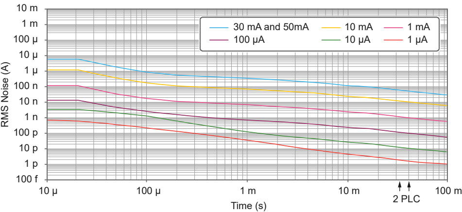
Figure 4. Current RMS Noise Versus Aperture Time 21, 22
