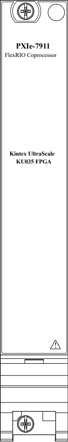
Figure 3. PXIe-7911 Front Panel
