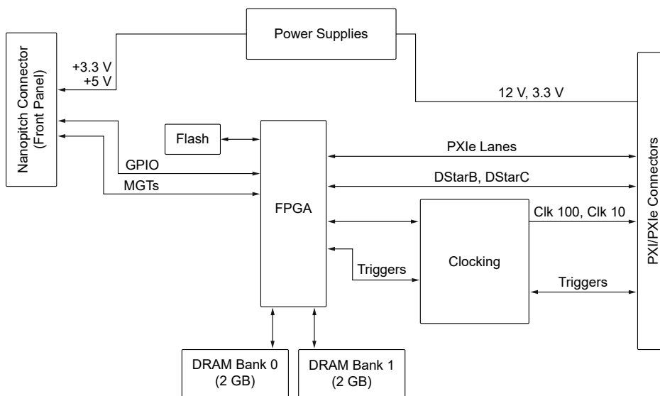
Figure 7. PXIe-7912 and PXIe-7915 Block Diagram
